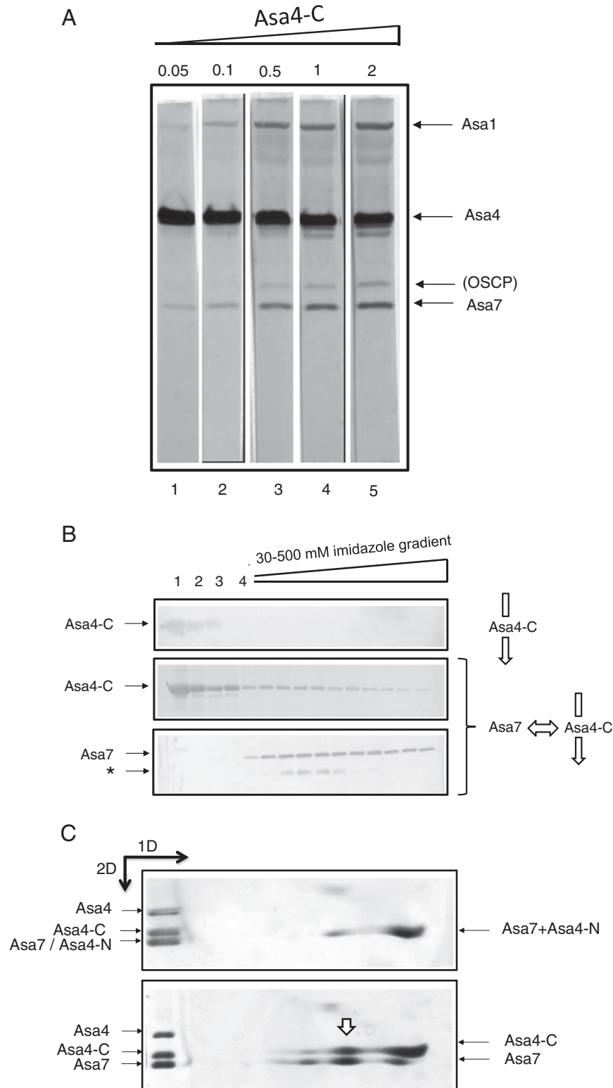
Fig. 3. Interaction of Asa4 fragments with Asa7. A) Far-Western analysis of Polytomella ATP synthase (25 \mu g of protein per lane) incubated for 4 h with increasing nanomoles of the isolated, recombinant Asa4-C fragment as indicated (in a 5 mL final volume), and then decorated with an anti-Asa4 antibody. B) Interaction of the Asa4-C fragment and Asa7 assayed by affinity chromatography. The crude extract containing the expressed Asa4-C fragment was loaded on a 1 mL HisTrap column containing no bound proteins (upper panel) or to which the Asa7 subunit, containing a 6His-tag, was previously bound (middle and lower panels). Western blot decorated with anti-Asa7 (lower panel) or anti-Asa4 (upper and middle panels) of the column fractions collected upon application of a 30 to 500 mM imidazole gradient. Lane 1, crude extract loaded on the column; lane 2, protein excluded from the column; lanes 3 and 4, proteins excluded from the column after washing with 30 mM imidazole. C) Identification of subcomplexes Asa4-N/Asa7 and Asa4-C/Asa7. One nanomole of each polypeptide was incubated together in a final volume of 50 \mu L and loaded onto 1D-BN-PAGE followed by 2D-Tricine-SDS-PAGE. Upper panel: a small amount of Asa7–Asa4-N subcomplex was formed in these conditions. Lower panel: A putative Asa4-C/Asa7 subcomplex is indicated with a white arrow. Three micrograms of each of the molecular mass markers, Asa4 (31.2 kDa), Asa4-C (14.9 kDa) and Asa7 (20.5 kDa) was loaded on the left-hand side of the gels.
